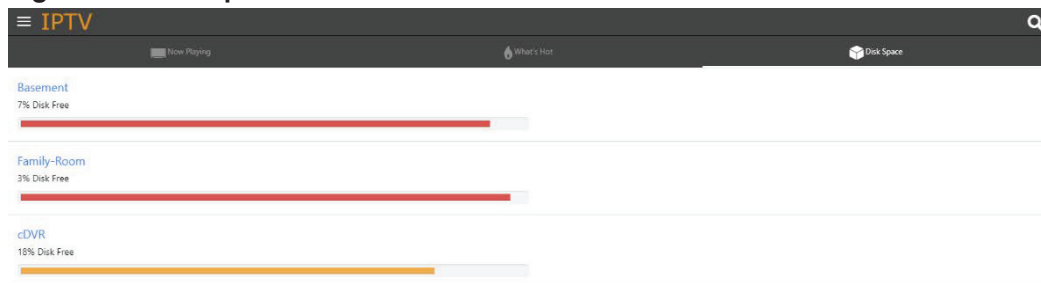
Figure 1-4 Disk Space
